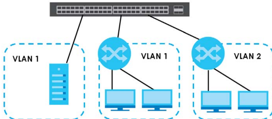
Figure 5 Shared Server Using VLAN Example
