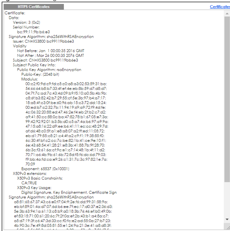
Figure 198 Management &gt; Maintenance &gt; Certificates &gt; HTTPS
